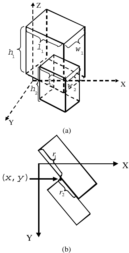
Figure 11 Parameters of two boxes standing on the ground surface and joined by common side. (a) side view; (b) vertical view
